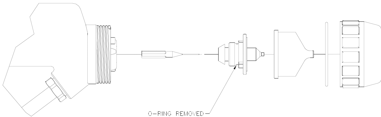
Figure 1 Vector Coded R90/R70 O-RING REMOVED DIAGRAM
