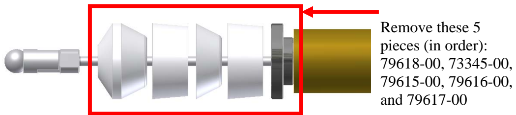
Old needle shaft assembly (79575-00) for use with old revision barrels
