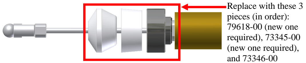
New needle shaft assembly (79970-00) for use with new revision barrels with tan insert
